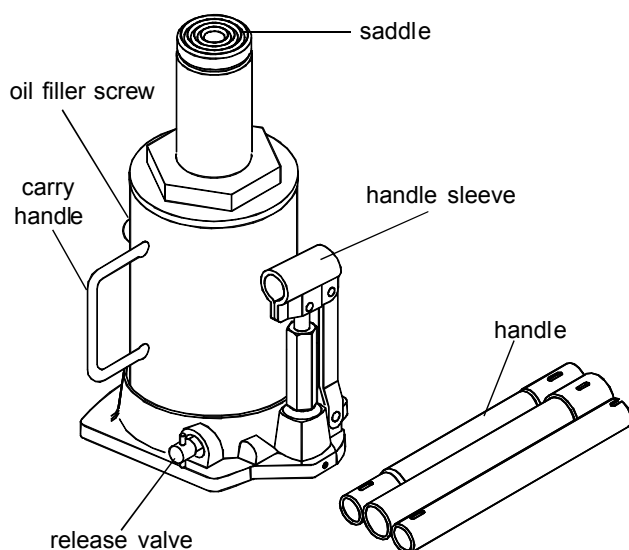
Figure 1 - 10300 Nomenclature
