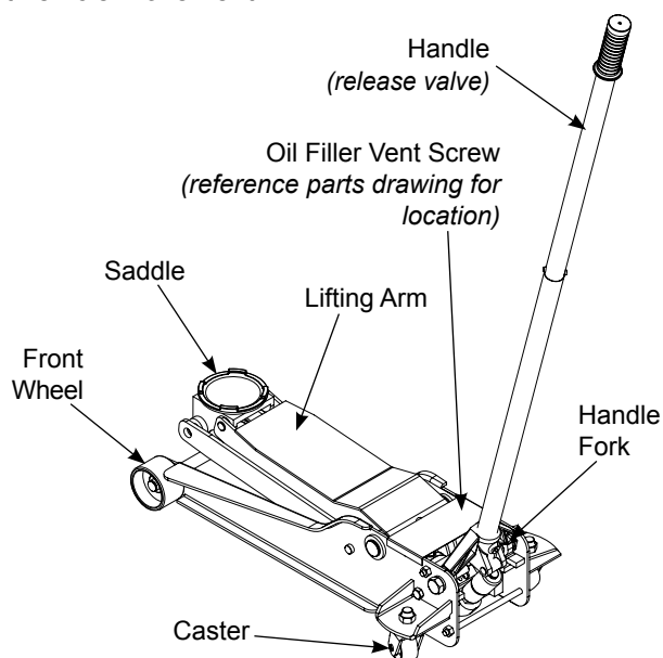
Figure 1 - Typical Jack Nomenclature
