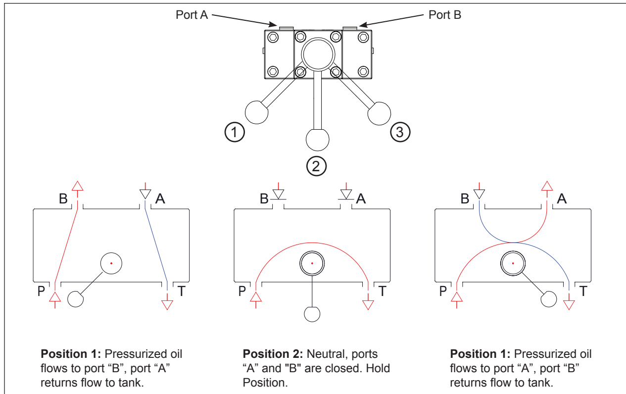
Figure 2 - Flowpath of the valve positions and operations
