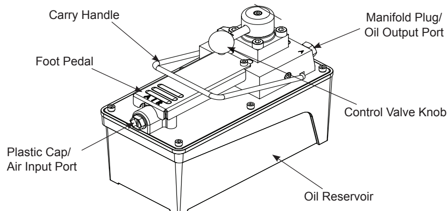
Figure 1 - Model PA1500M Components
